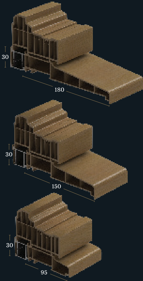
RANGE OF CILLS
