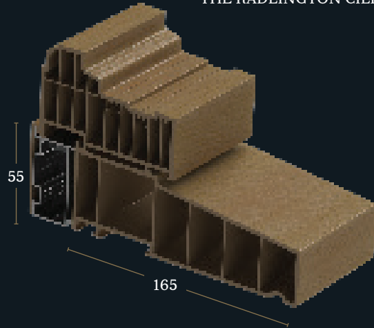
THE RADLINGTON CILL
